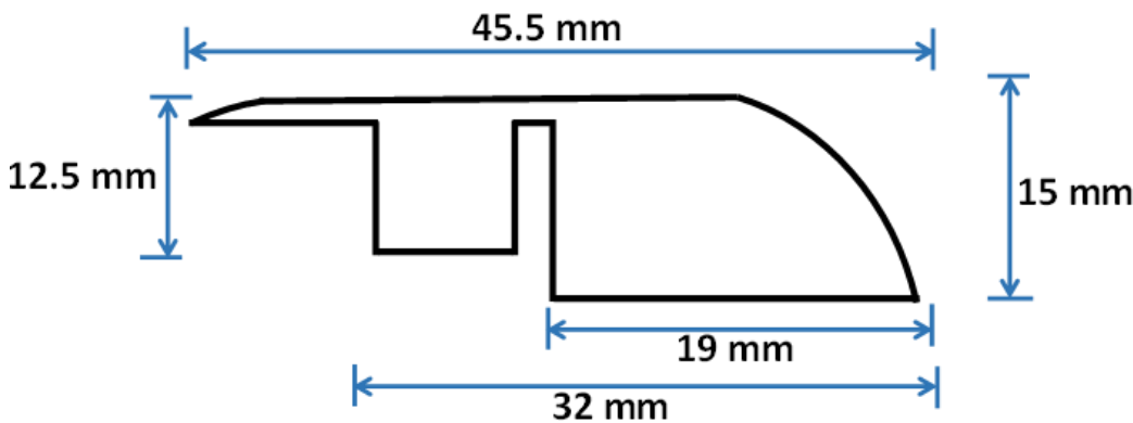
LAMINATE REDUCER (OVERLAP)
