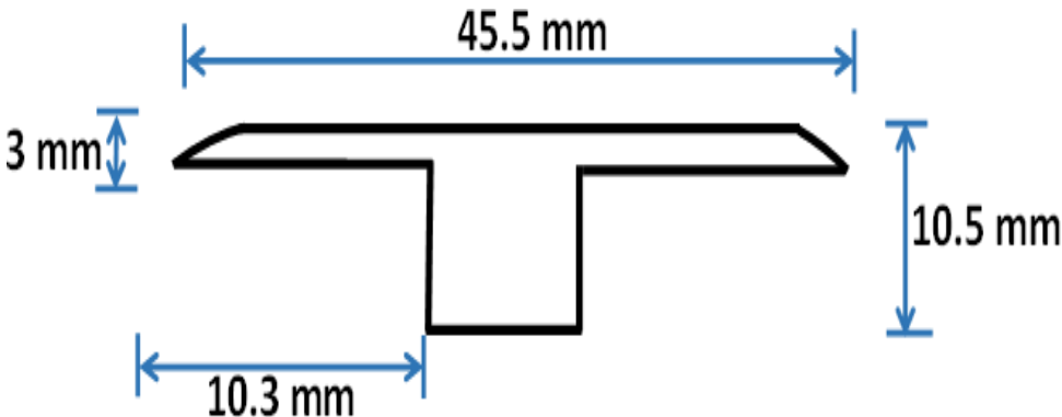
LAMINATE T-MOULDING (OVERLAP)
