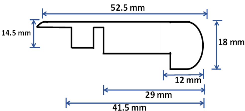
LAMINATE STAIR-NOSE (OVERLAP)
