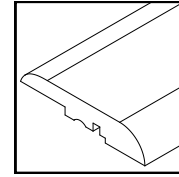
Reducer 2400 × 45 × 12 mm
