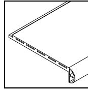
Stair Nosing † 2400 × 55 × 18 mm
