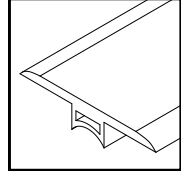
T-Moulding 2400 × 45 × 12 mm
