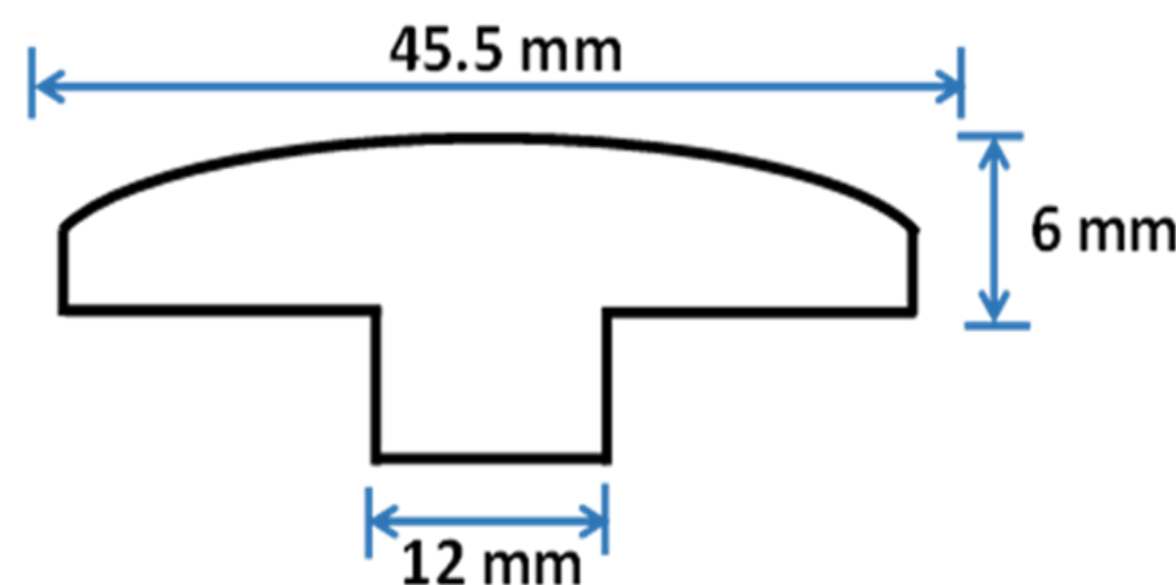
ENG HWD T-MOLDING OVERLAP
